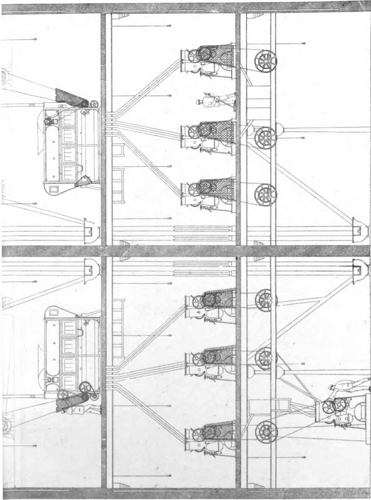
W. VERNON & SONS' NEW FLOUR MILLS, BIRKENHEAD DOCKS. CROSS SECTION OF THE ROLLING AND DRESSING MACHINERY FLOORS.
